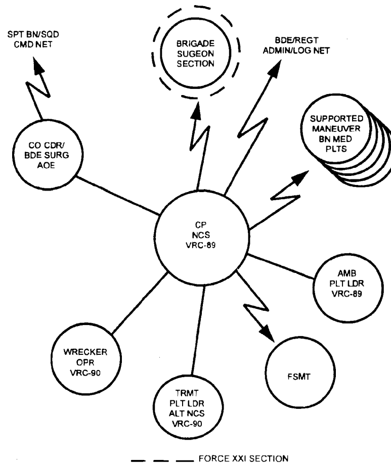
Figure 3-7. Medical company/tr troop command FM net/brigade medical operations net.
