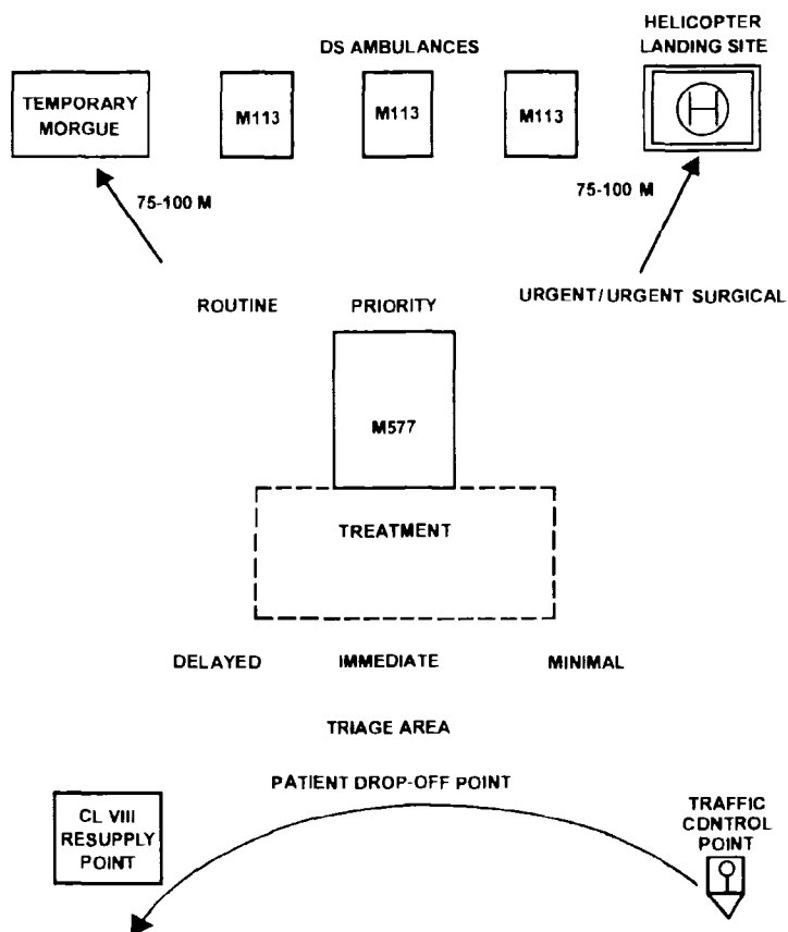
Figure 2-8. Layout of a battalion aid station (heavy).
