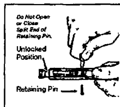
Figure 071-311-2025-12. Removing the firing pin retaining pin
