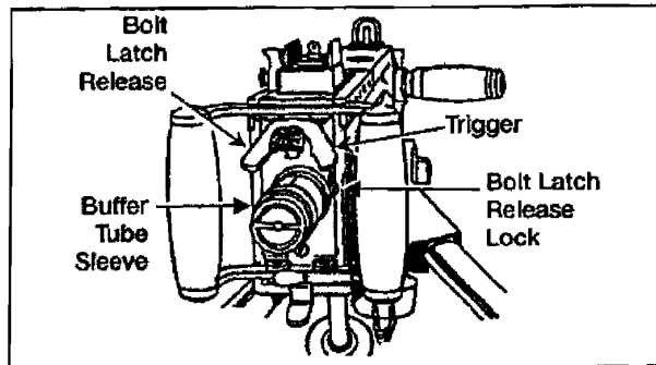
Figure 071-022-0001-3. Releasing the bolt latch
