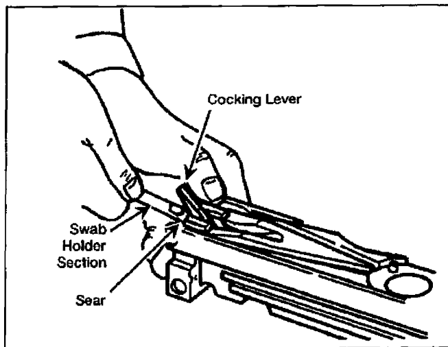
Figure 071-022-0001-10. Releasing the firing pin spring
