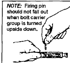
Figure 071-311-2025-30. Placing the firing pin retaining pin
