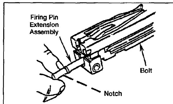
Figure 071-022-0001-31. Installation of the firing pin extension assembly
