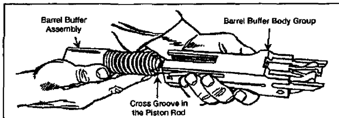
Figure 071-022-0001-18. Removal of the barrel buffer assembly
