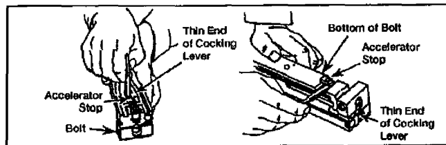
Figure 071-022-0001-13. Removal of the accelerator stop
