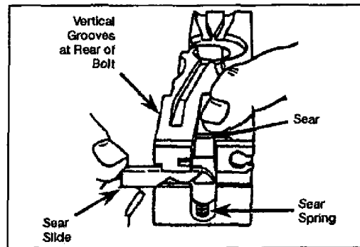
Figure 071-022-0001-32. Installation of the sear side
