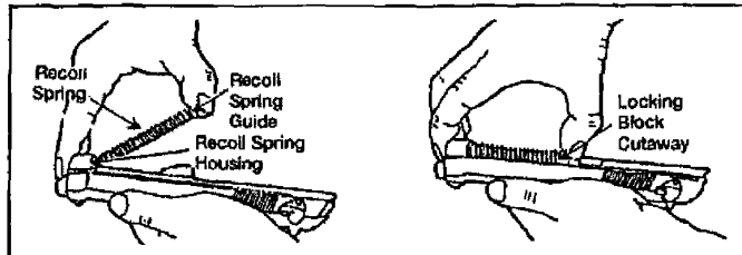
Figure 071-004-0001-7. Insertion of the recoil spring and guide
