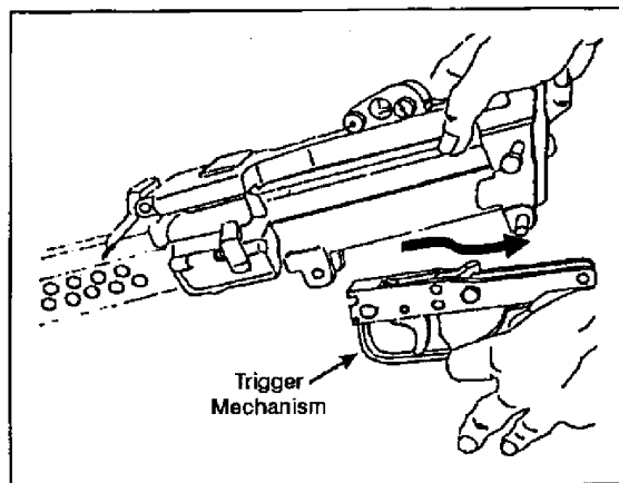
Figure 071-312-4025-12. Removal of the trigger mechanism
