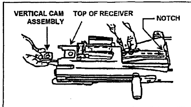
Figure 071-030-0001-22. Engaging the vertical cam assembly.
