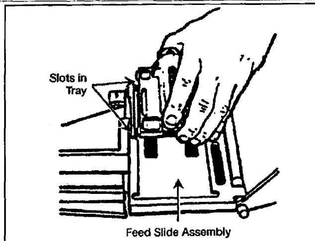
Figure 071-030-0001-8. Removal of the feed slide assembly.
