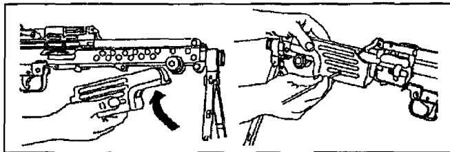
Figure 071-312-4025-23. Replacement of the handguard
