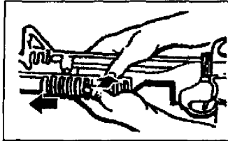
Figure 071-311-2125-4. Unlocking and opening the M203 barrel
