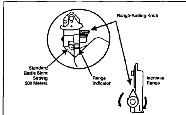
Figure 071-054-0001-6. Adjusting the rear sight
