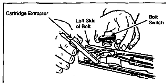
Figure 071-022-0001-9. Removal of the cartridge extractor and bolt
