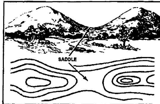
Figure C-8. Saddle
