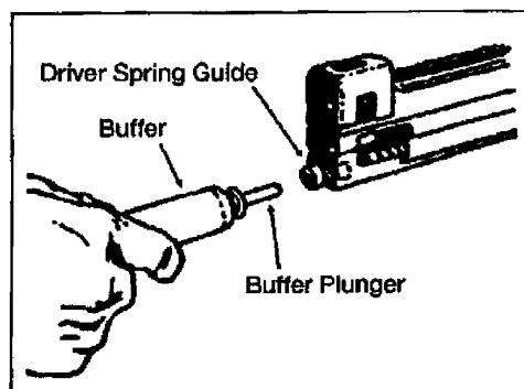
Figure 071-312-3025-3. Buffer
