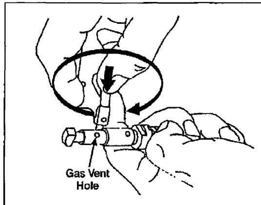
Figure 071-312-4025-15. Cleaning the gas vent hole
