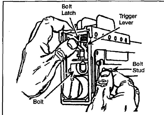
Figure 071-022-0001-7. Unlatching the bolt
