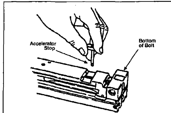
Figure 071-022-0001-33. Attachment of the accelerator stop
