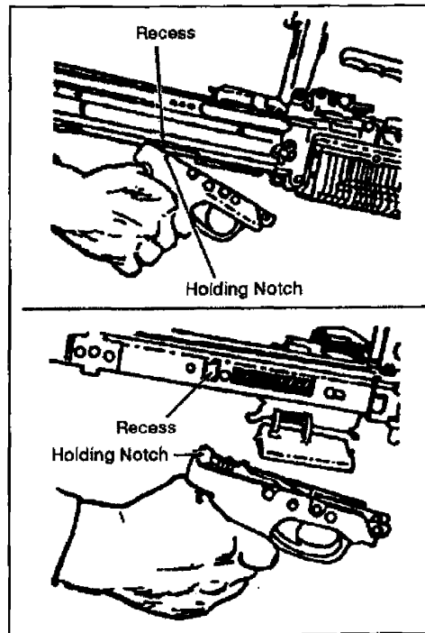
Figure 071-312-3025-8. Trigger mechanism group
