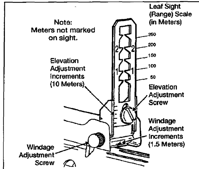
Figure 071-311-2130-4. Leaf sight
