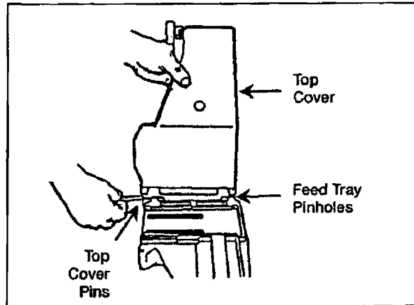
Figure 071-030-0001-20. Attachment of the top cover assembly
