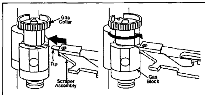
Figure 071-312-4025-9. Insertion of the scraper assembly
