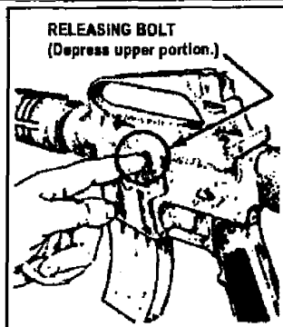
Figure 071-311-2027-7. Bolt catch.
