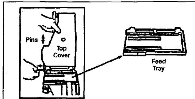
Figure 071-030-0001-9. Removal of the top cover assembly and feed tray
