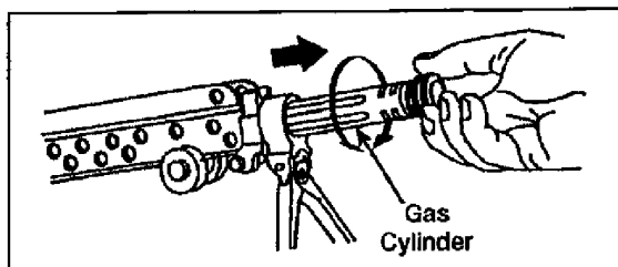
Figure 071-312-4025-13. Removal of the gas cylinder
