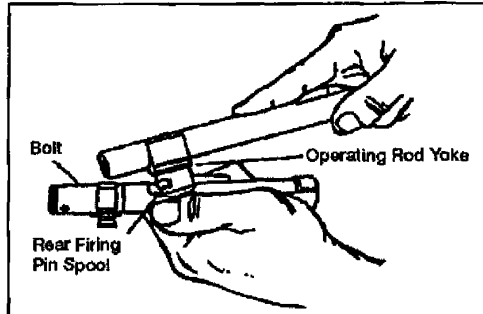
Figure 071-312-3025-13. Rear of operating rod yoke positioned against rear firing pin spool
