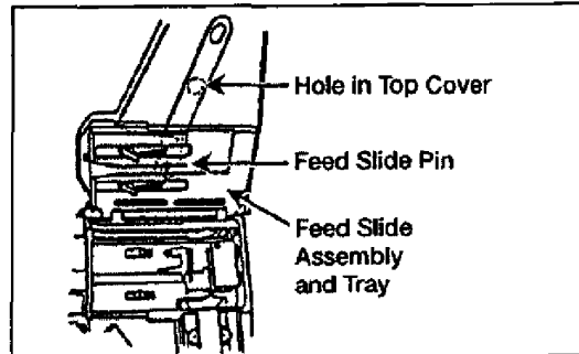
Figure 071-030-0001-21. Engaging the secondary drive lever
