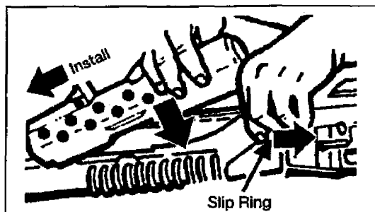
Figure 071-311-2125-9. Installing the handguard
