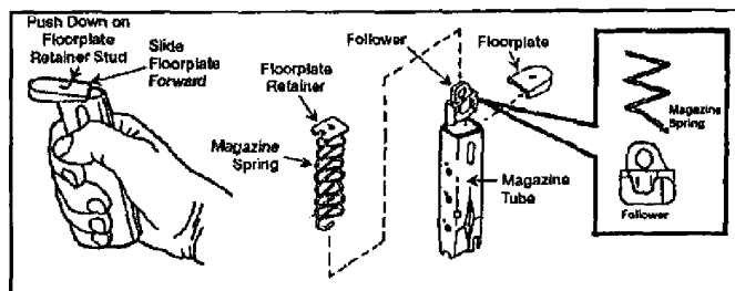
Figure 071-004-0001-4. Disassembly of the magazine
