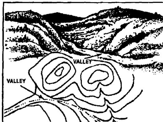
Figure C-7. Valley
