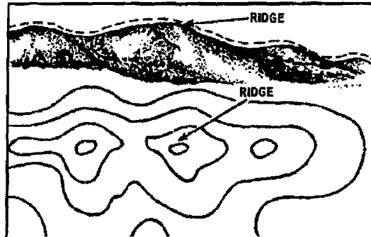
Figure C-6. Ridge
