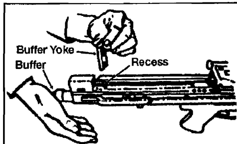
Figure 071-312-3025-2. Buffer yoke
