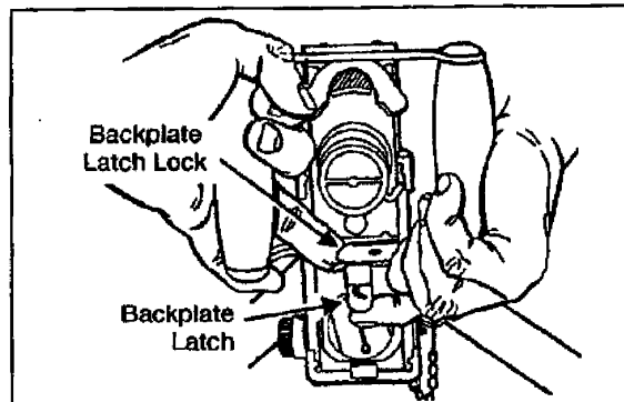
Figure 071-022-0001-4. Removal of the backplate
