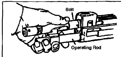
Figure 071-312-3025-14. Operating rod and bolt
