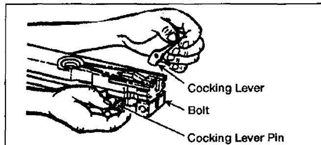
Figure 071-022-0001-35. Attachment of the cocking lever
