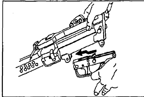
Figure 071-312-4025-27. Replacement of trigger mechanism
