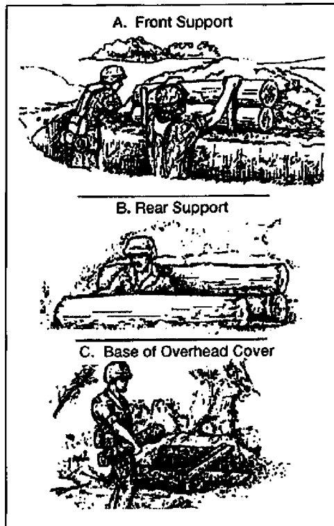
Figure 071-326-5703-5. Constructing overhead cover (1)
