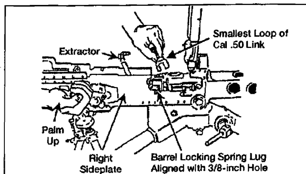
Figure 071-022-0001-2. Alignment of the lug
