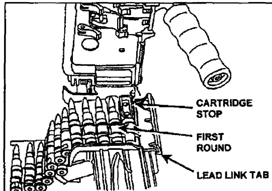
Figure 071-312-4027-4. Link belt in feed tray
