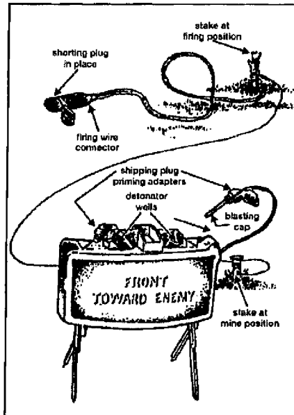
Figure 071-325-4425-11. Arming the mine
