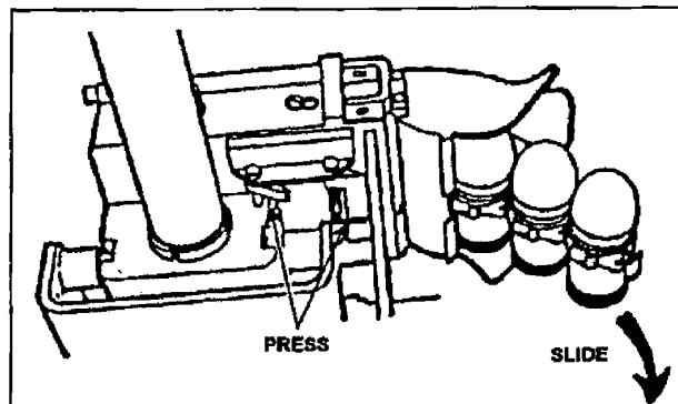
Figure 071-030-0006-2. Removal of Linked Rounds from the Feeder
