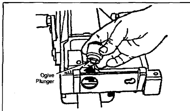
Figure 071-030-0001-11. Removal of the ogive plunger
