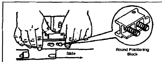
Figure 071-030-0001-12. Removal of the round positioning block
