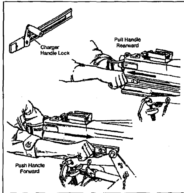
Figure 071-030-0005-4. Charging the MK19 machine gun
