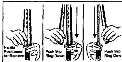
Figure 071-311-2025-5. Removing the handguards
