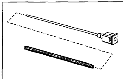
Figure 071-312-4025-3. Removal of the spring
