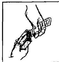
Figure 071-311-2025-42. Removing the magazine spring and the follower
