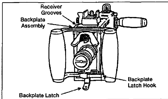
Figure 071-022-0001-42. Installation of the backplate assembly
