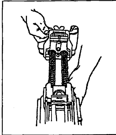
Figure 071-030-0001-3. Removal of bolt and backplate assembly
