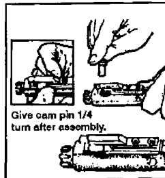
Figure 071-311-2025-28. Replacing the bolt cam pin
