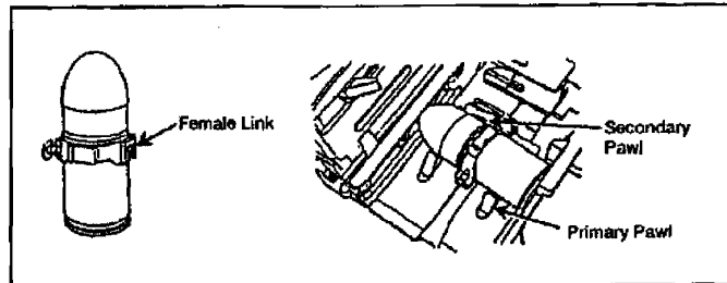
Figure 071-030-0005-1. Insertion of first round through feed throat
