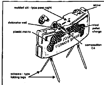
Figure 071-325-4425-5. Placing and aiming the mine
