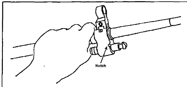
Figure 071-312-4025-24. Replacement of the gas regulator
