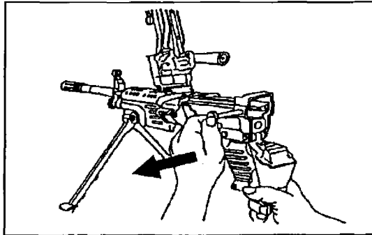
Figure 071-312-4025-1. Rear opening of the receiver
