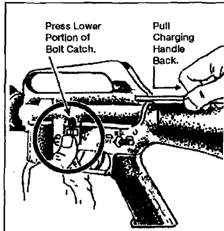
Figure 071-311-2025-2. Locking the bolt open
