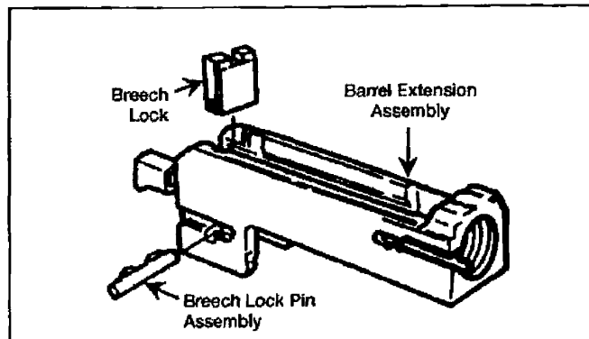
Figure 071-022-0001-26. Assembly of the barrel extension assembly (1) Install breechblock lock with beveled edge up and to the front of barrel extension assembly.
