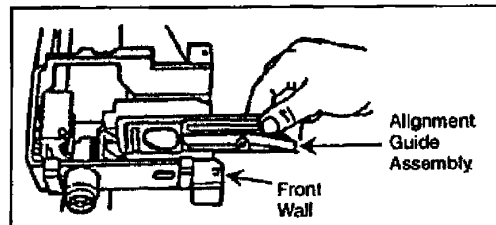
Figure 071-030-0001-18. Insertion of the alignment guide assembly
