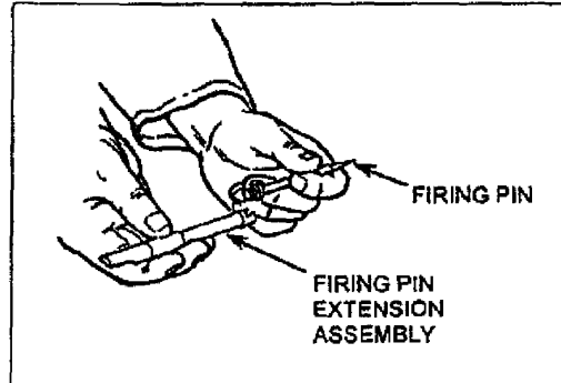
Figure 071-022-0001-30. Attachment of the firing pin to the firing pin extension assembly
