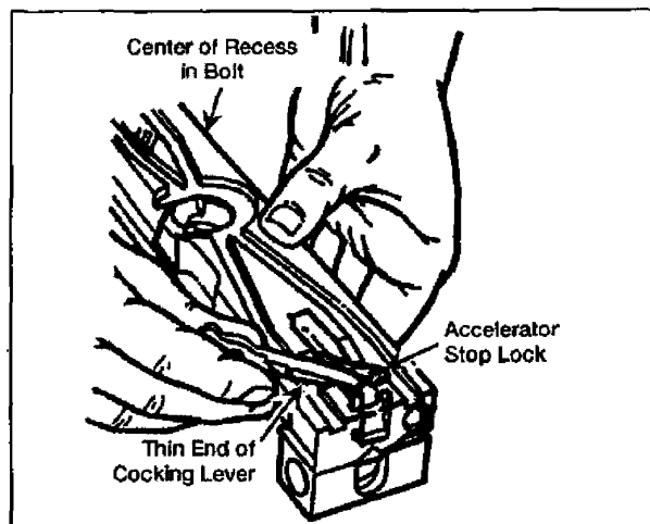
Figure 071-022-0001-12. Removal of the accelerator stop lock
