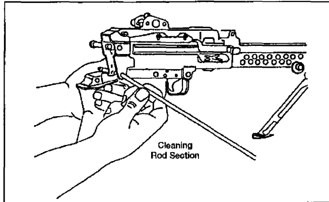
Figure 071-312-4025-11. Removal of the buttstock and buffer assembly
