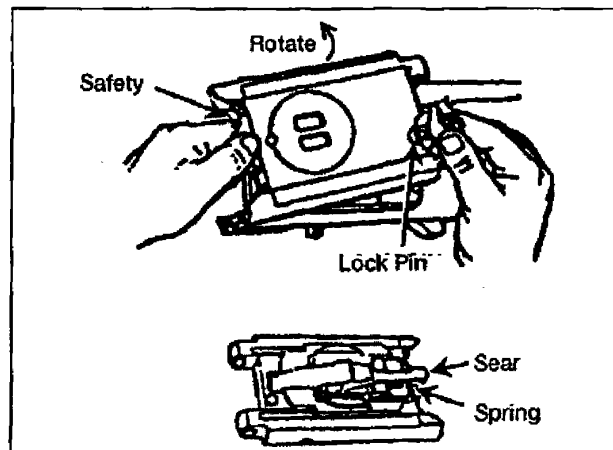
Figure 071-030-0001-14. Removal of the receiver sear assembly
