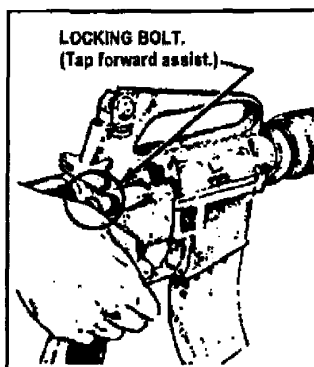
Figure 071-311-2027-8. Forward assist.
