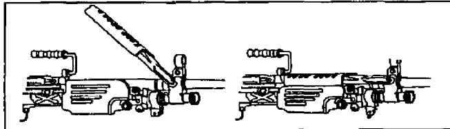
Figure 071-312-4025-35. Replacement of the heat shield assembly
