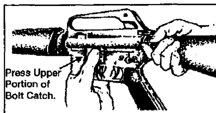
Figure 071-311-2025-4. Releasing the bolt
