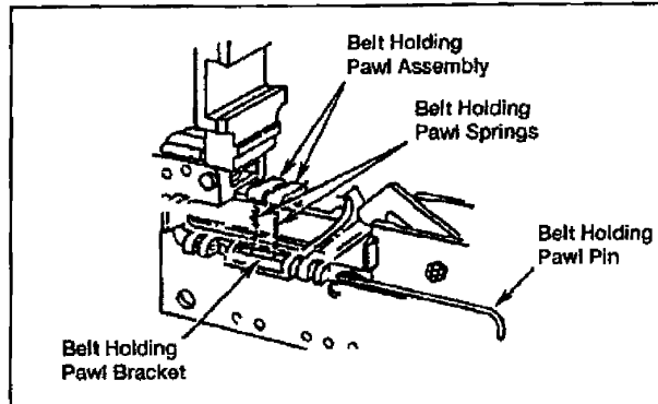
Figure 071-022-0001-25. Installation of the belt holding pawl assembly c. Assemble barrel extension (figure 071-022-0001-26).
