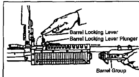
Figure 071-312-3025-11. Barrel locking lever
