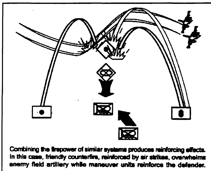
Figure 4-9. Reinforcing Effects
