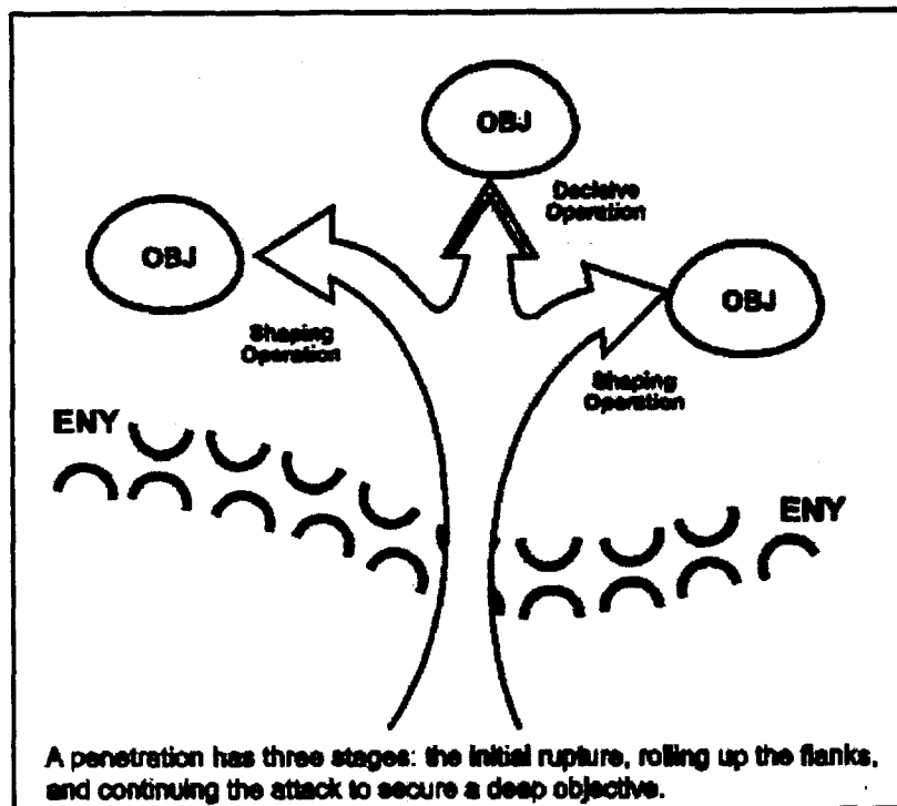
Figure 7-5. Penetration
