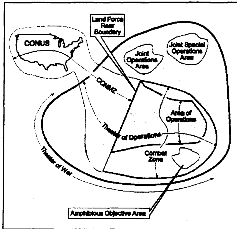
Figure 4-3. Theater Organization
