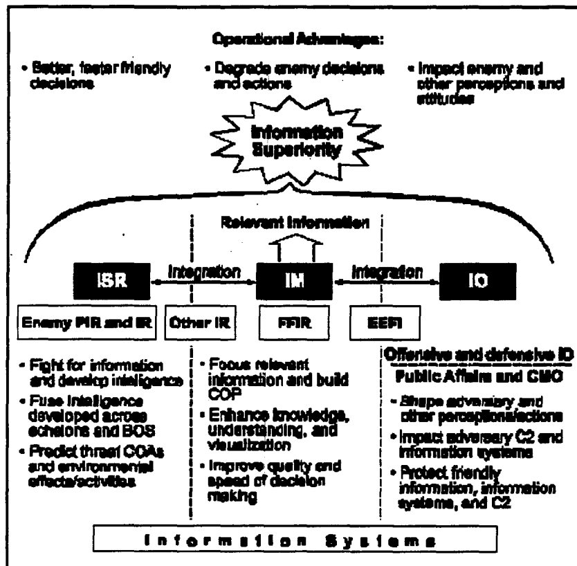
Figure 11-1. Information Superiority
