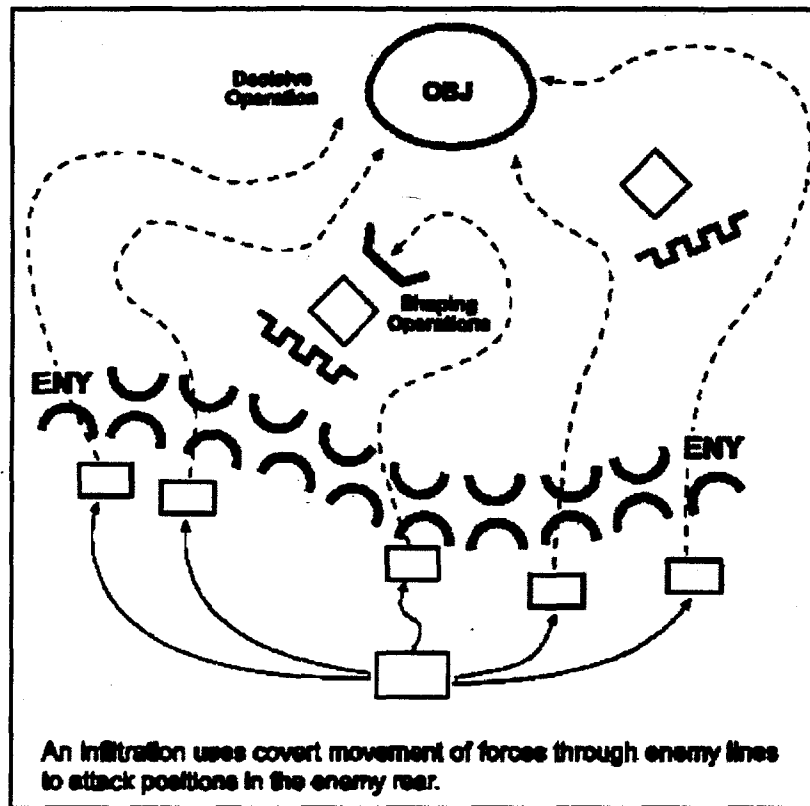
Figure 7-4. Infiltration
