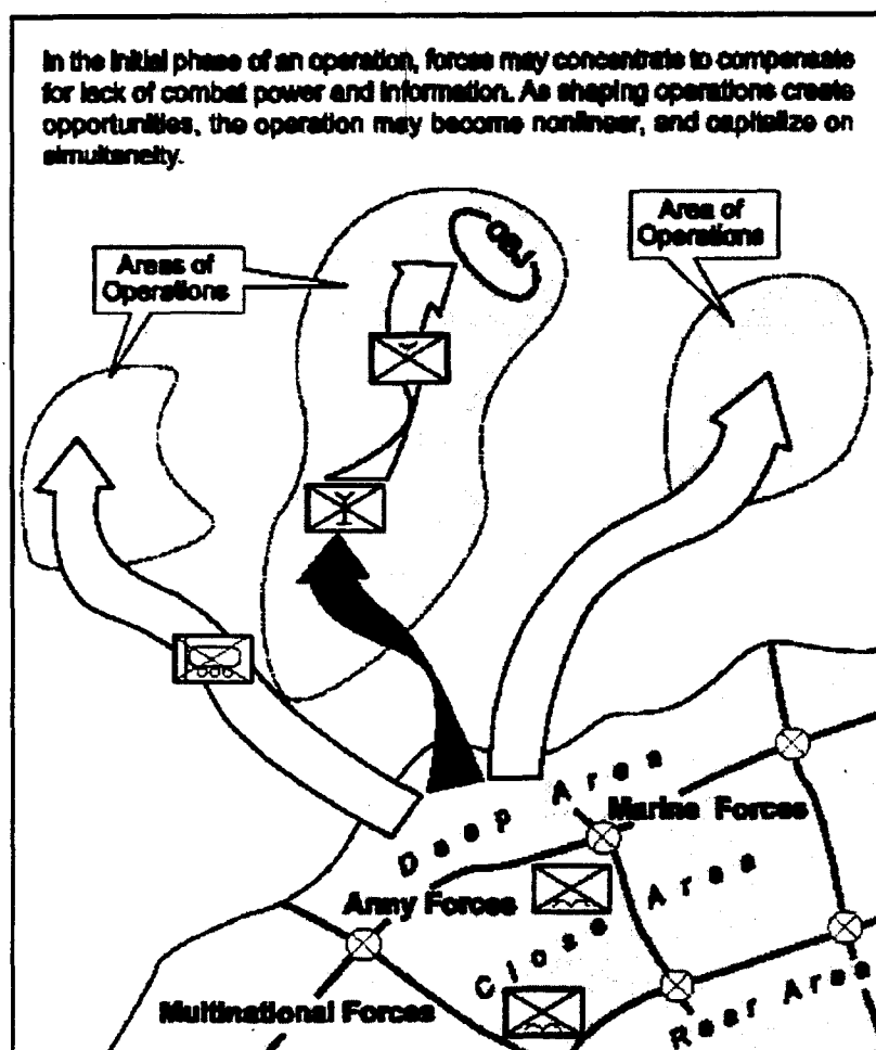
Figure 6-2. Linear and Nonlinear Combinations
