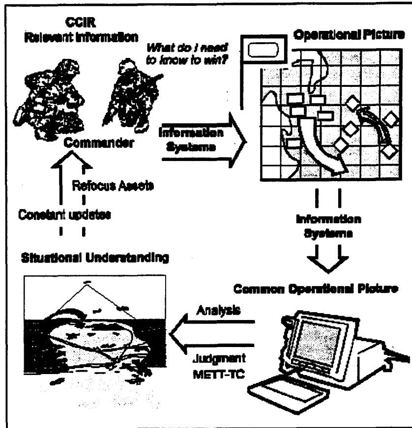
Figure 11-3. Situational Understanding
