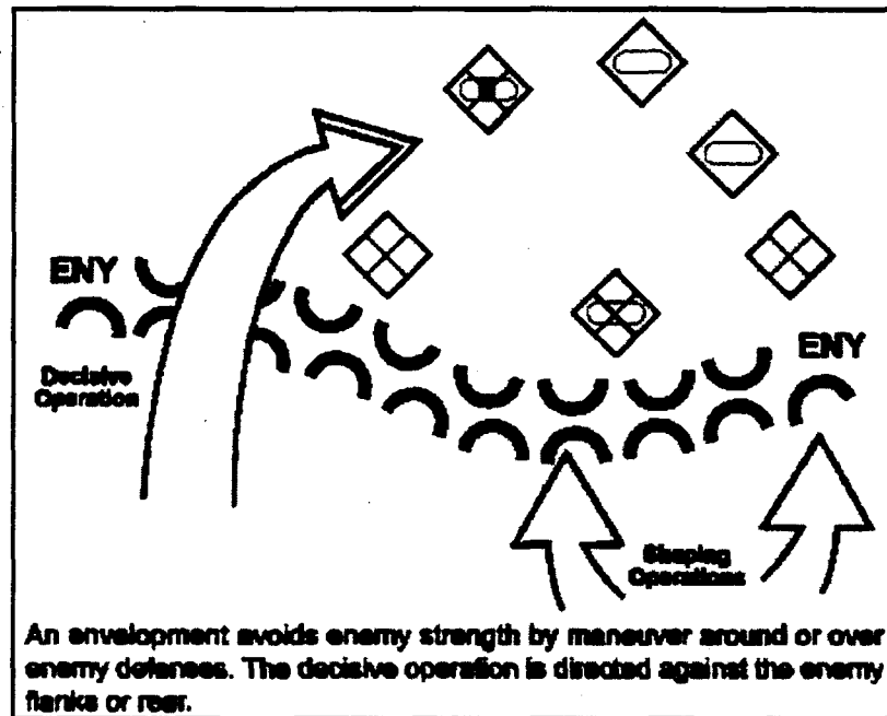
Figure 7-2. Envelopment
