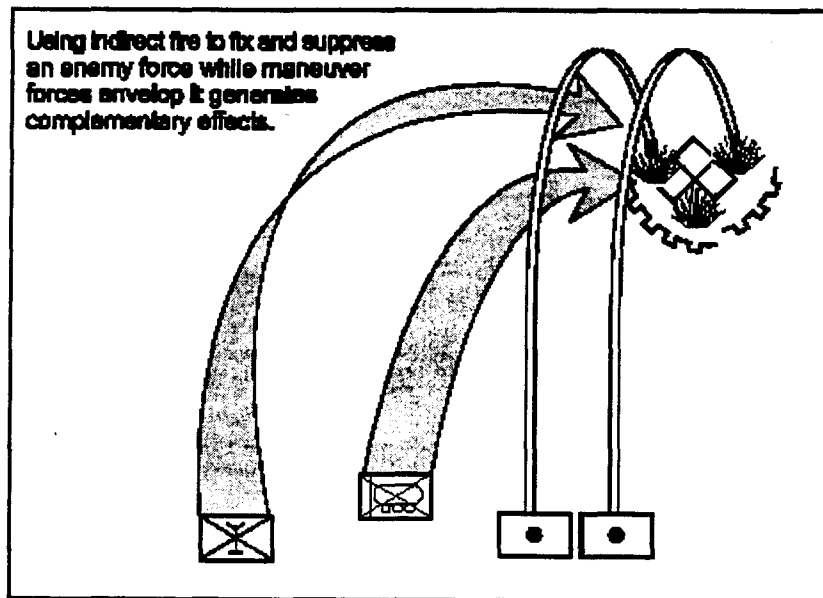
Figure 4-8. Complementary Effects
