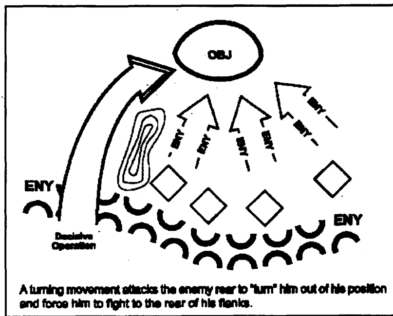
Figure 7-3. Turning Movement
