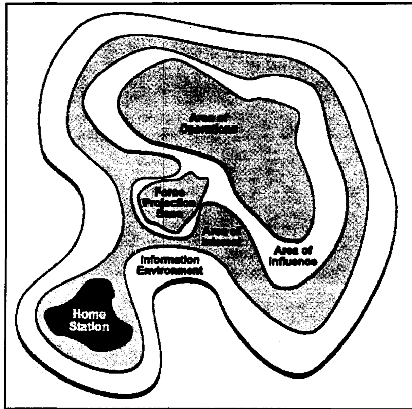
Figure 4-5. Battlespace Components
