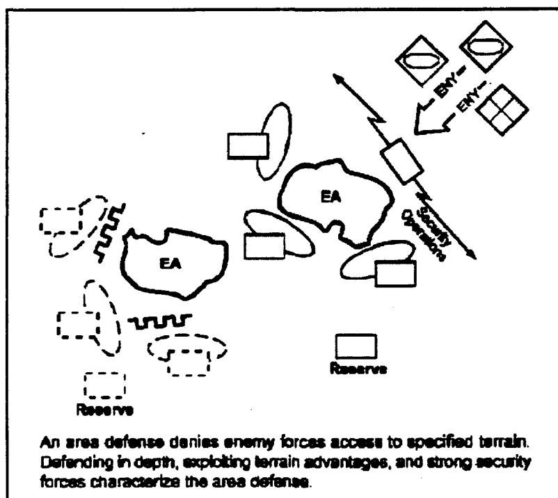
Figure 8-2. Area Defense
