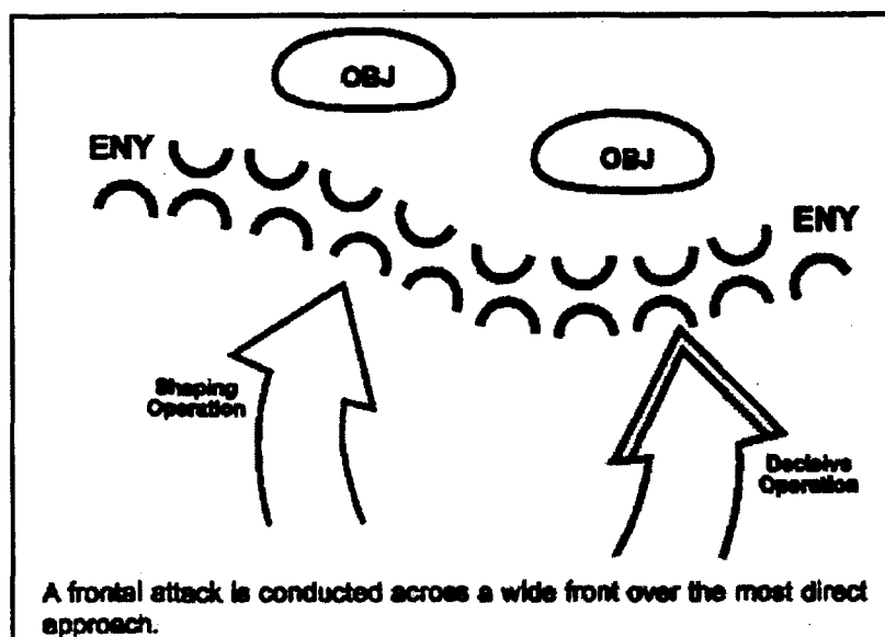
Figure 7-6. Frontal Attack
